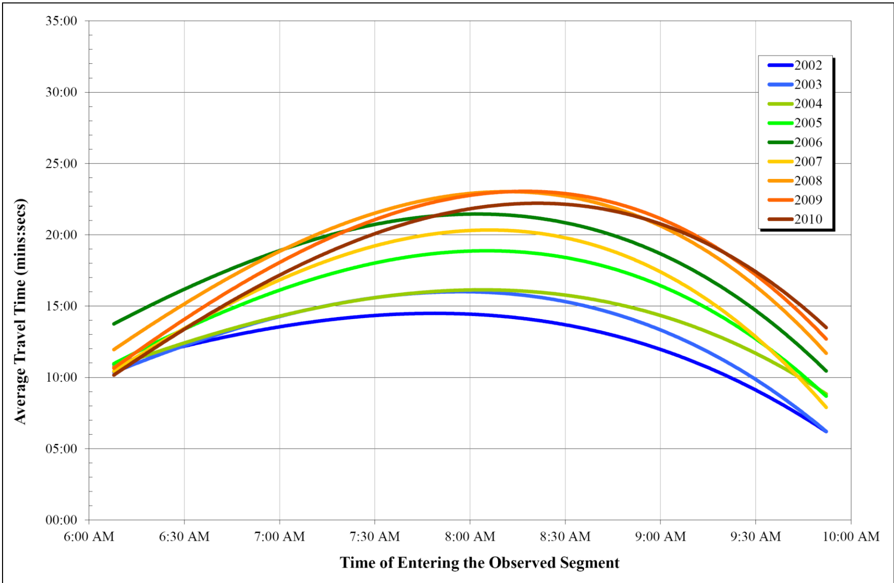
FIGURE 7 Southeast Expressway Travel Times Northbound General-Purpose Lanes (6:00 AM–10:00 AM)
