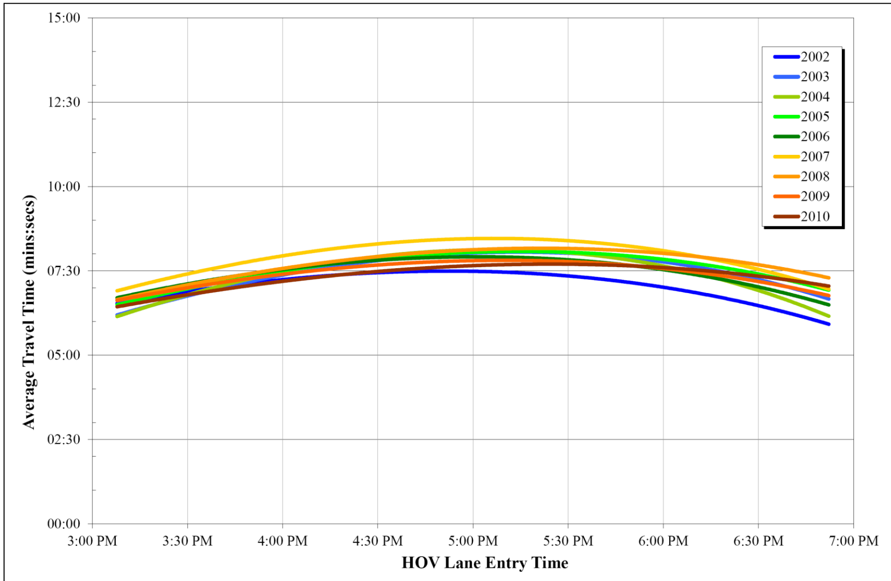
FIGURE 8 Southeast Expressway Travel Times Southbound HOV Lane (3:00 PM–7:00 PM)
