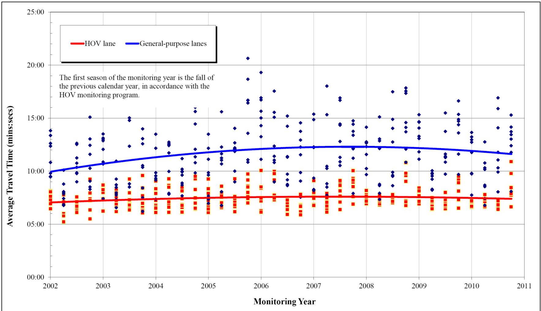
FIGURE 3 Southeast Expressway Travel Times Southbound Travel Lanes (3:00 PM–7:00 PM)
