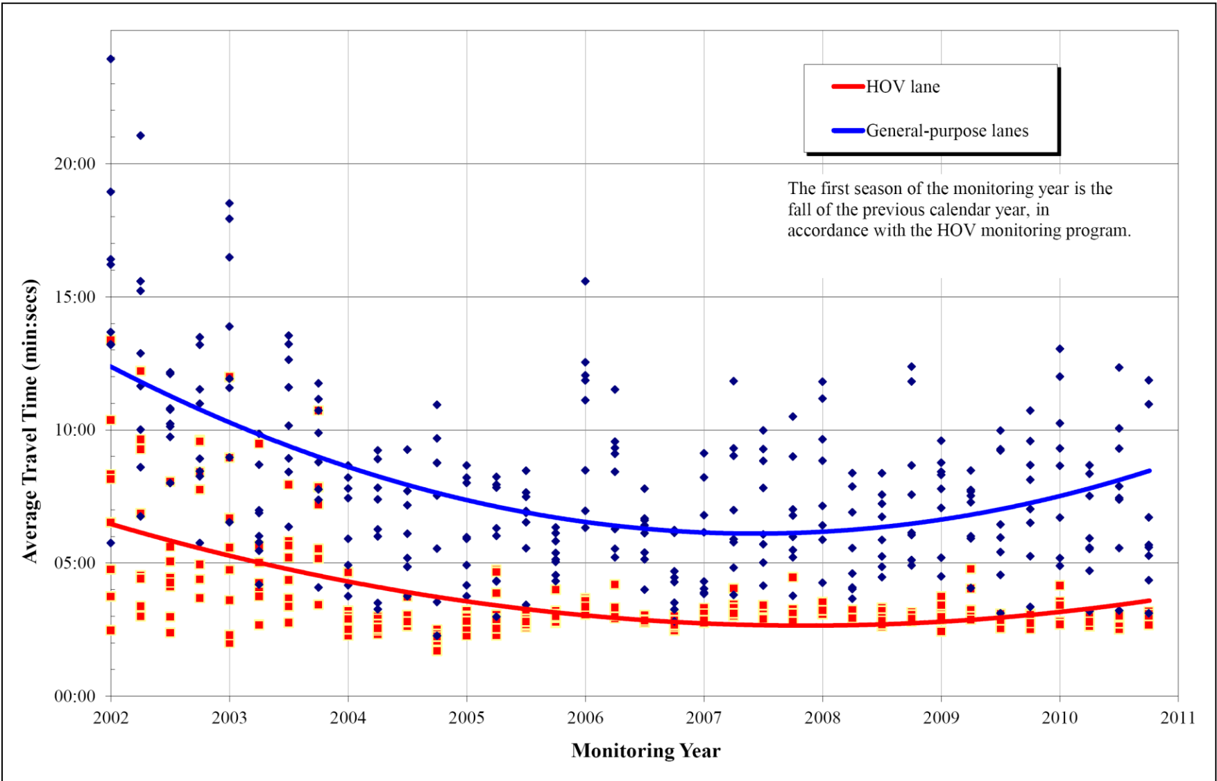
FIGURE 1 I-93 North Travel Times Southbound Travel Lanes (6:00 AM–10:00 AM)
