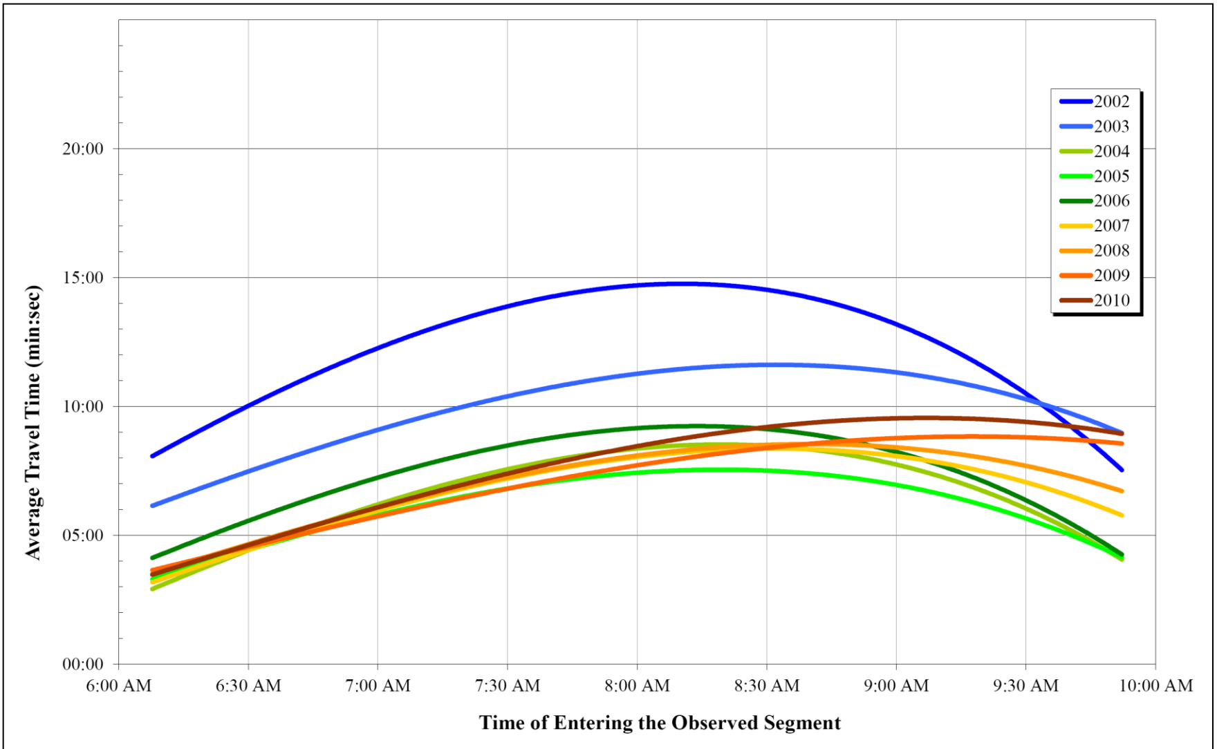
FIGURE 5 I-93 North Travel Times Southbound General-Purpose Lanes (6:00 AM–10:00 AM)
