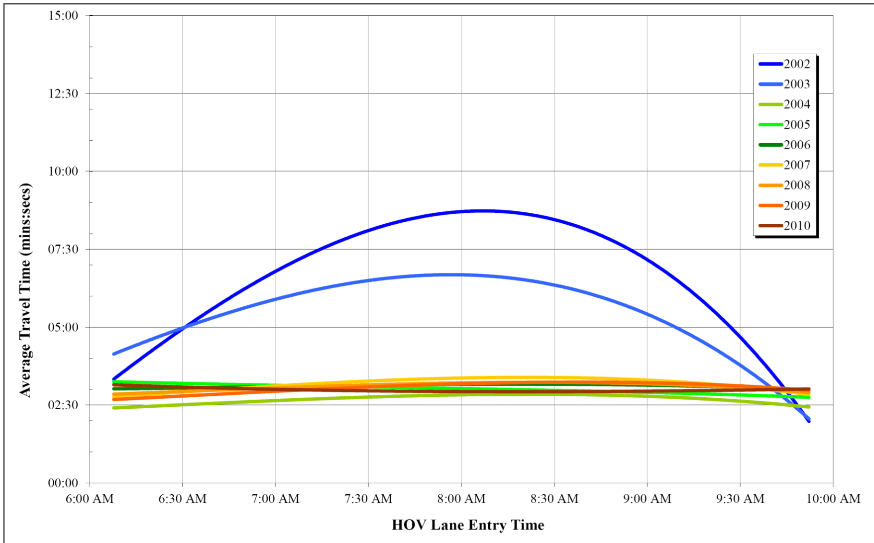
FIGURE 4 I-93 North Travel Times Southbound HOV Lane (6:00 AM–10:00 AM)
