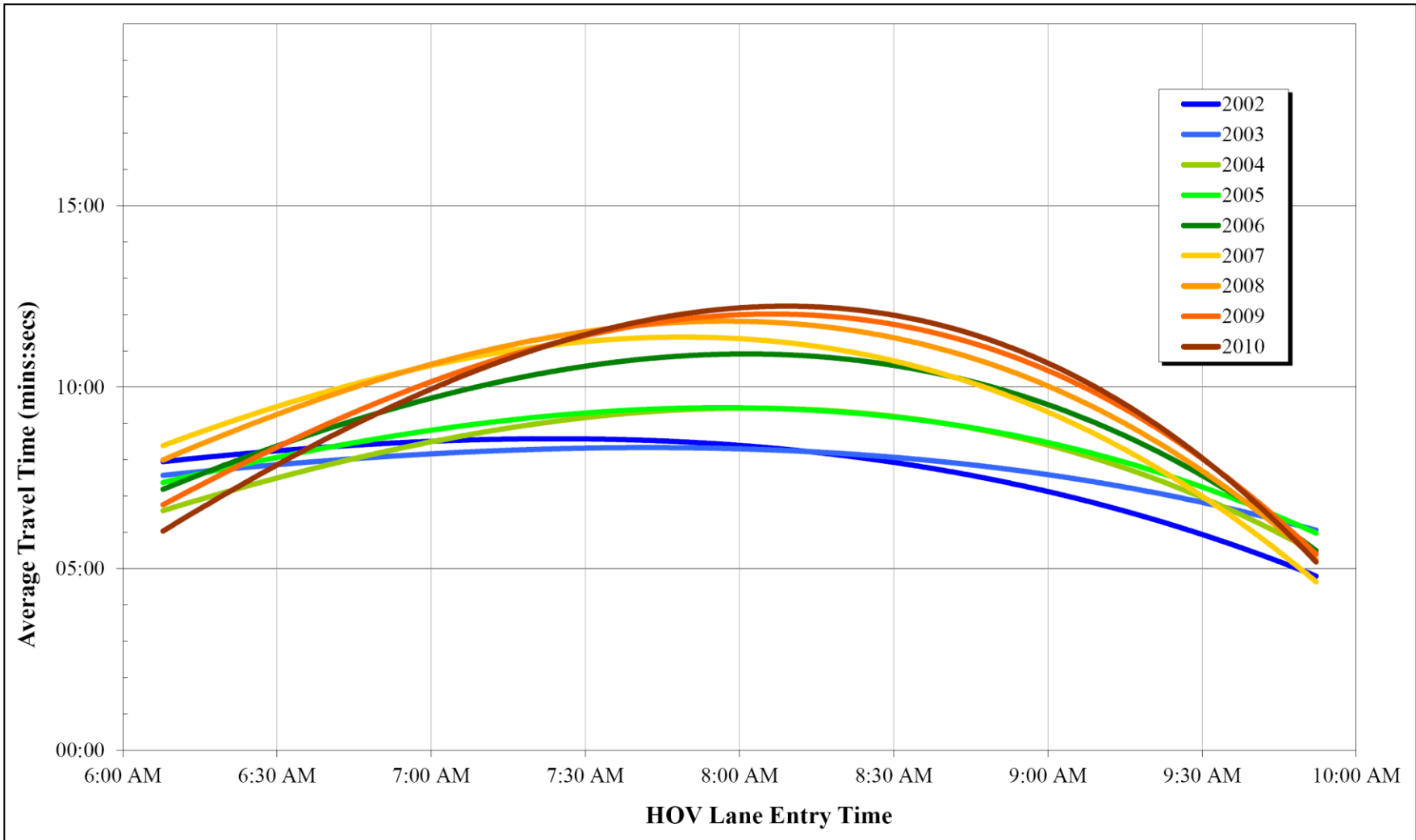
FIGURE 6 Southeast Expressway Travel Times Northbound HOV Lane (6:00 AM–10:00 AM)
