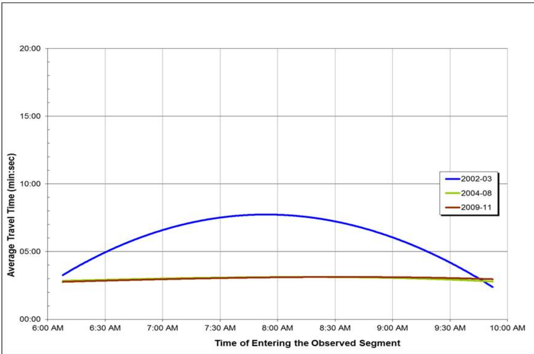
FIGURE 4 I-93 North Travel Times: Southbound HOV Lane, AM Peak Period, 2002-11
